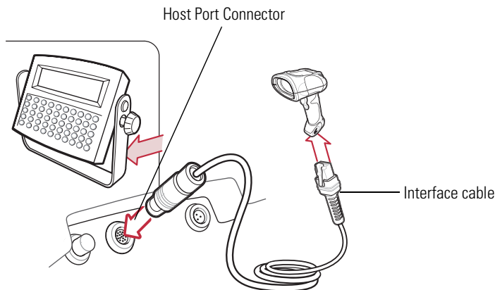
Figure 10-1. Scanner Emulation Connection
