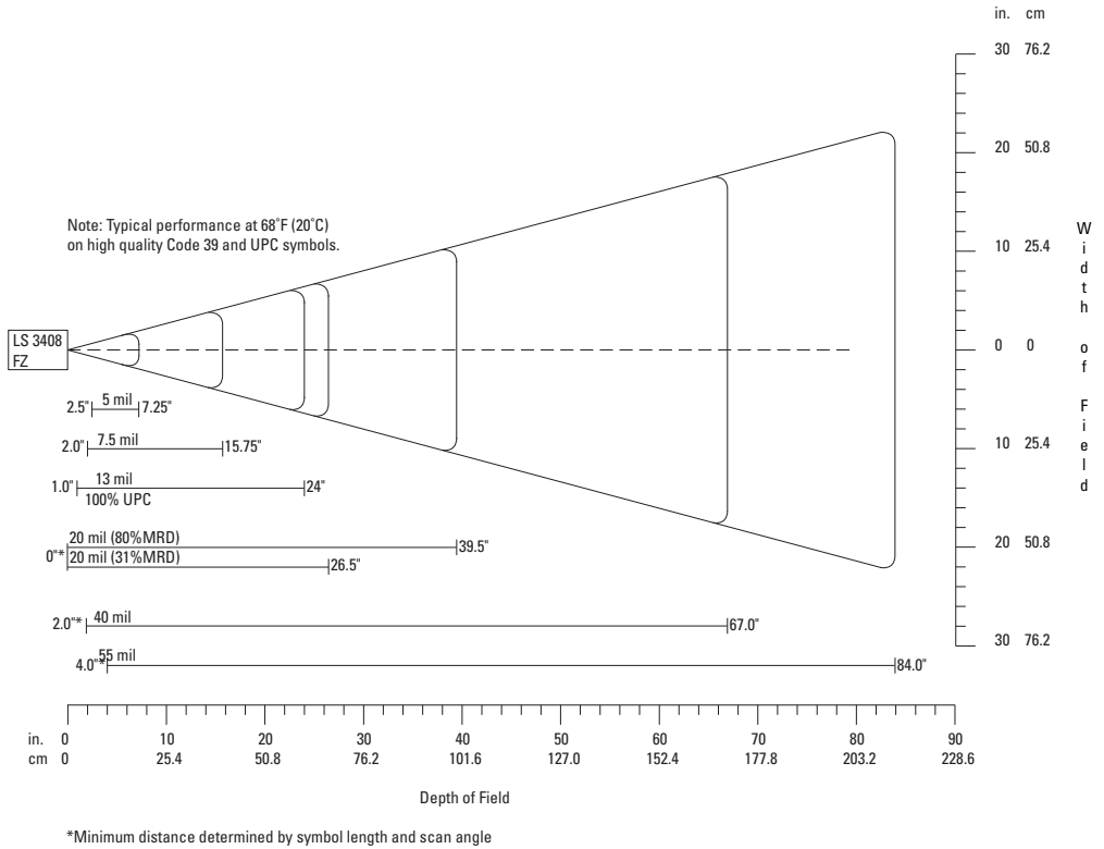
Figure 2-5. LS 3408-FZ Decode Zone
