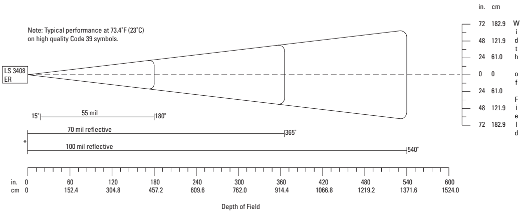
Figure 2-6. LS 3408-ER Decode Zone
