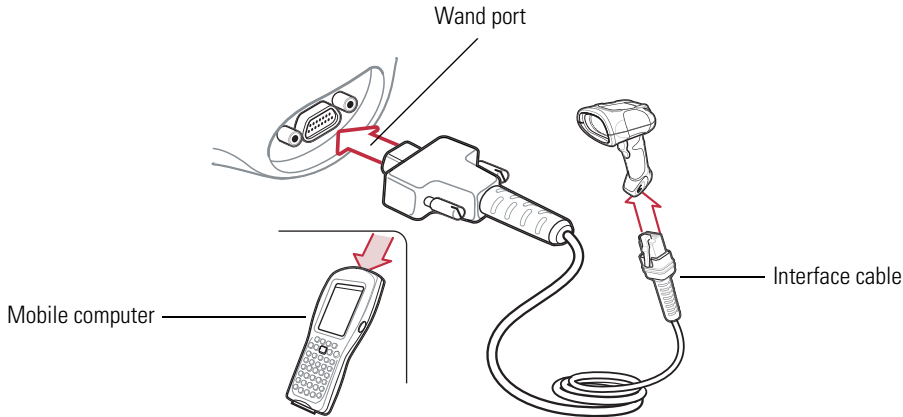
Figure 9-1. Wand Emulation Connection
